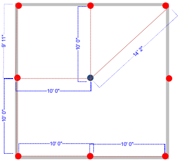
20' x 20' pole Tent - Pole Placement
